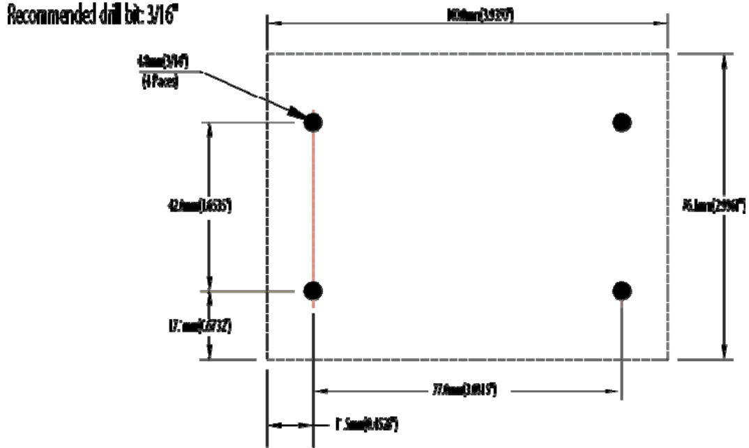
Figure 2 Stencil of moles to mount enclosure directly to a surface without brackets
